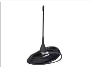
GMAE4255 Panel mount antenna with 380-430 MHz frequency range and TETRA.
