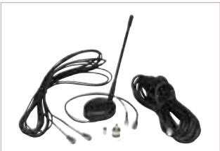
GMAE4290 Combined TETRA and GPS antenna for digital car kit operating in the 380-430MHz frequency range - includes duplexer and DC adapter. Compatible with car kit FTN6307.
