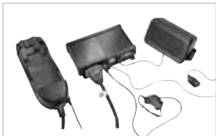
GMLN4687 Hands-free digital car kit including cradle, junction box, external speaker, remote microphone, velcro-mount PTT and cable 12V to 24V compatibility.
