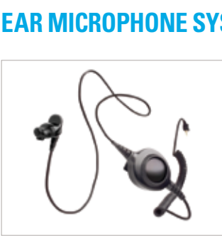
PMLN5561 Bone Conduction Ear Microphone with in-line large push-to-talk with protective ring. Speak softly and be heard. Suitable also in high noise environment when ear muffs are worn over the ear microphones.
