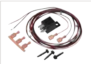
GKN6272 External alarm relay and cable.
